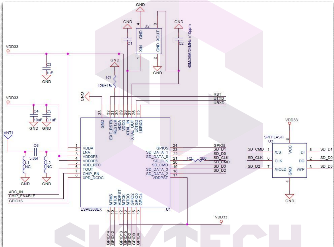
Figure 4 Schematics of ESP-12F WiFi Module
